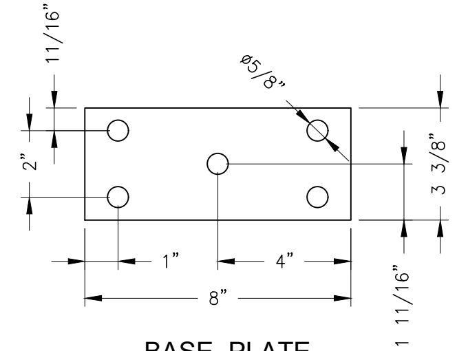
BASE PLATE HOLE LAYOUT
