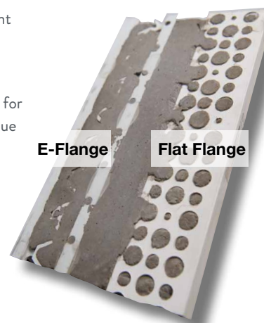
Photo illustrates E-Flange embedment vs. standard flange embedment at the backside of the flanges.
